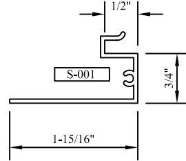
"B" HEAD/JAMB PANNING B (JAMB)
