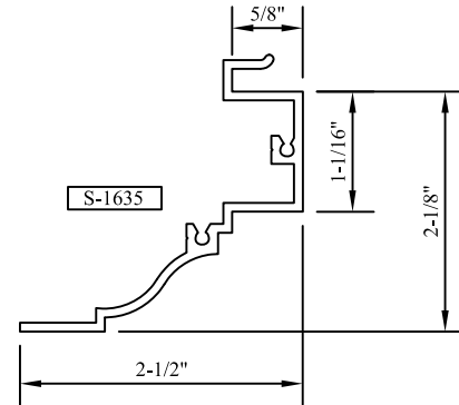
"N" HEAD/JAMB PANNING N (JAMB)
