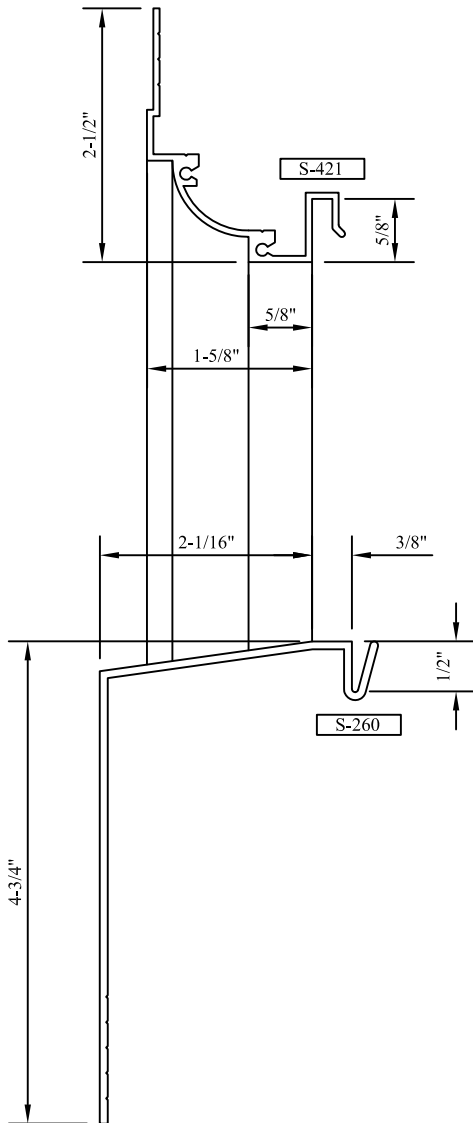
"L" SILL PANNING L (SILL)
