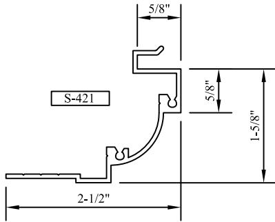
"AA" HEAD/JAMB PANNING AA (JAMB)
