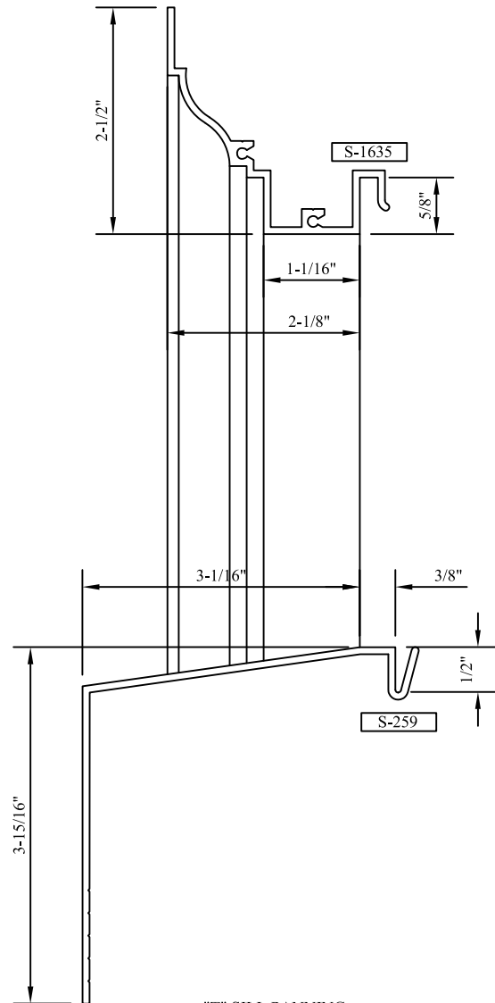
"T" SILL PANNING T (SILL)
