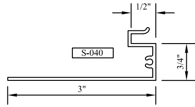
"E" HEAD/JAMB PANNING E (JAMB)
