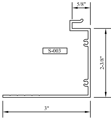
"D" HEAD/JAMB PANNING D (JAMB)
