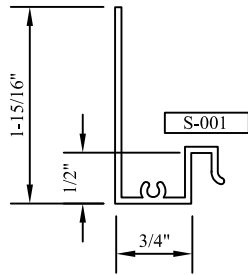
"B" HEAD/JAMB PANNING B
