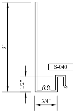
"E" HEAD/JAMB PANNING E
