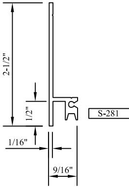
"HT" HEAD/JAMB PANNING HT
