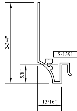
"PP" HEAD/JAMB PANNING PP
