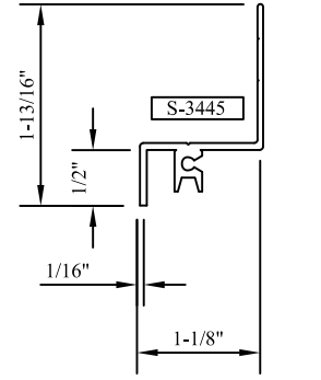
"NF" HEAD/JAMB PANNING NF
