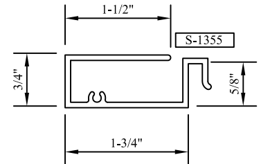
"IR" HEAD/JAMB PANNING IR
