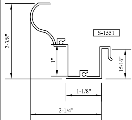
"TT" HEAD/JAMB PANNING TT
