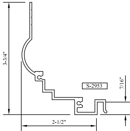
"DD" HEAD/JAMB PANNING DD
