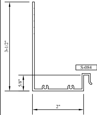
"L" HEAD/JAMB PANNING L
