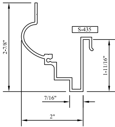
"DD" HEAD/JAMB PANNING DD
