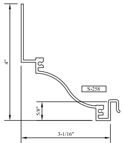
"T" HEAD/JAMB PANNING T
