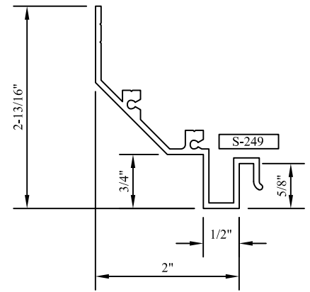
"O" HEAD/JAMB PANNING O
