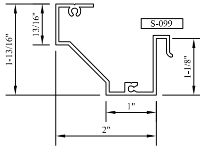
"P" RETURN HEAD/JAMB PANNING PR
