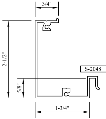
"EC" HEAD/JAMB PANNING EC
