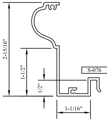
"J" RETURN HEAD/JAMB PANNING JR
