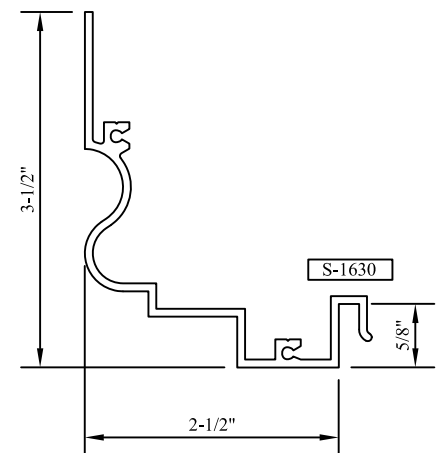
"WW" HEAD/JAMB PANNING WW
