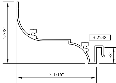
"P1" HEAD/JAMB PANNING P1
