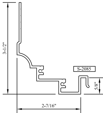
"DC" HEAD/JAMB PANNING DC
