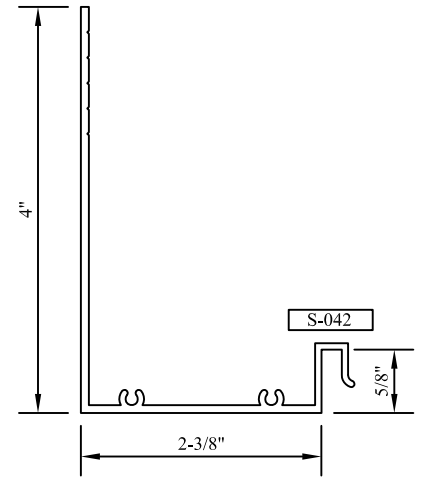
"D-MOD" HEAD/JAMB PANNING DM
