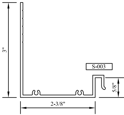
"D" HEAD/JAMB PANNING D
