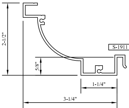
"AR" HEAD/JAMB PANNING AR
