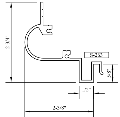
"V" HEAD/JAMB PANNING V
