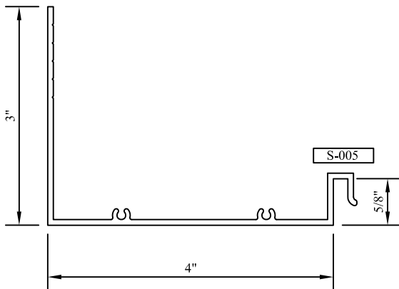
"C" HEAD/JAMB PANNING C
