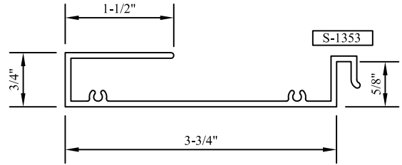
"SR" HEAD/JAMB PANNING SR
