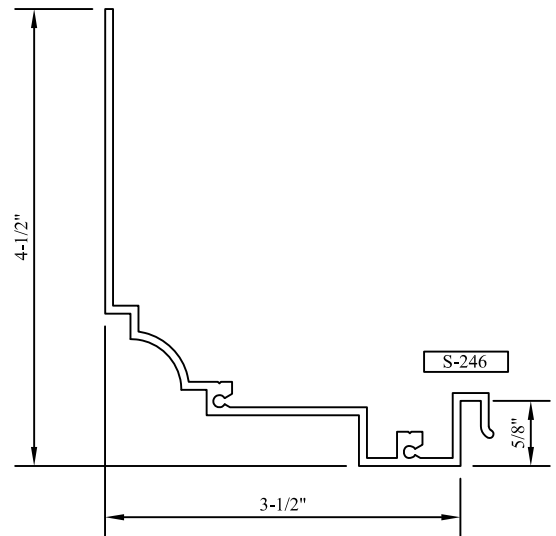
"Z" HEAD/JAMB PANNING Z
