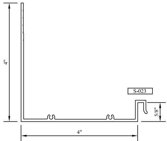
"C" MODIFIED HEAD/JAMB PANNING CM
