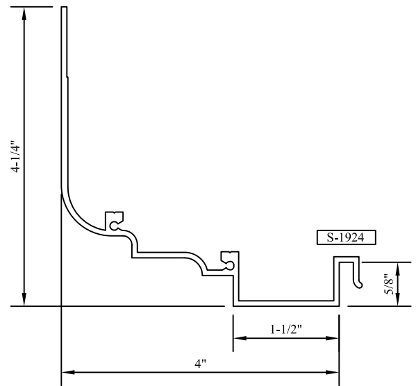
"M2" HEAD/JAMB PANNING M2
