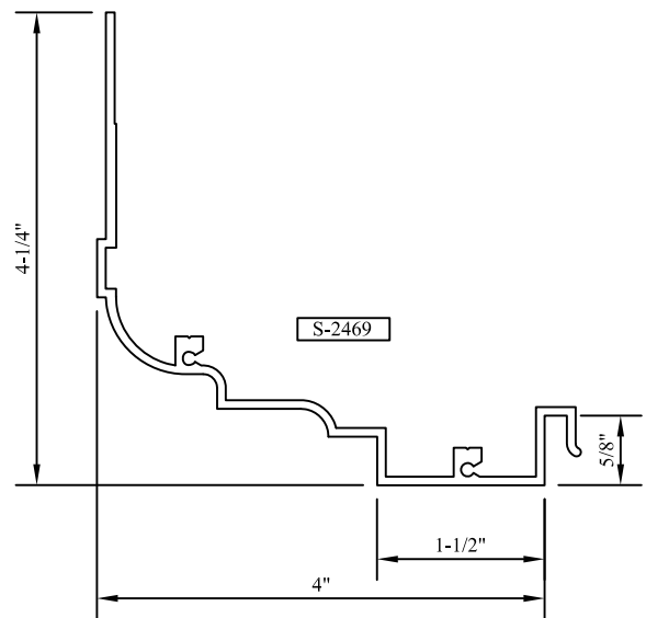
"MB" HEAD/JAMB PANNING MB
