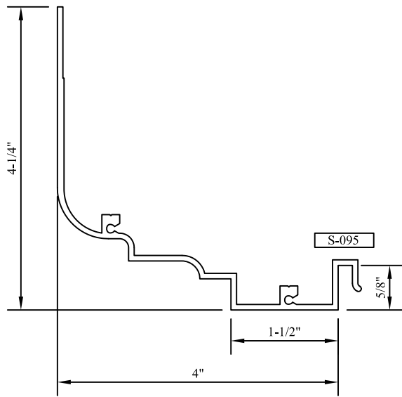
"M" HEAD/JAMB PANNING M
