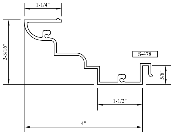
"MR" RETURN HEAD/JAMB PANNING MR
