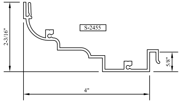
"MC" HEAD/JAMB PANNING MC
