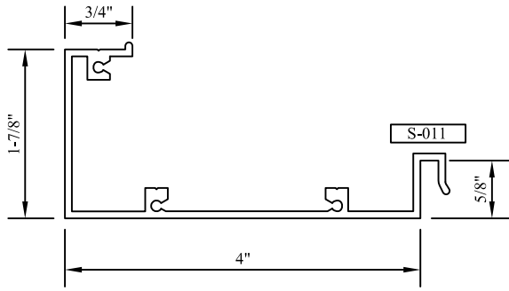
"C" RETURN HEAD/JAMB PANNING CR
