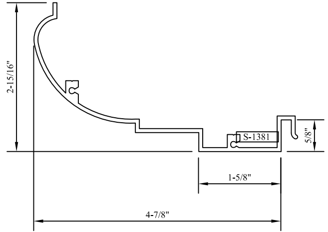
"NN" HEAD/JAMB PANNING NN
