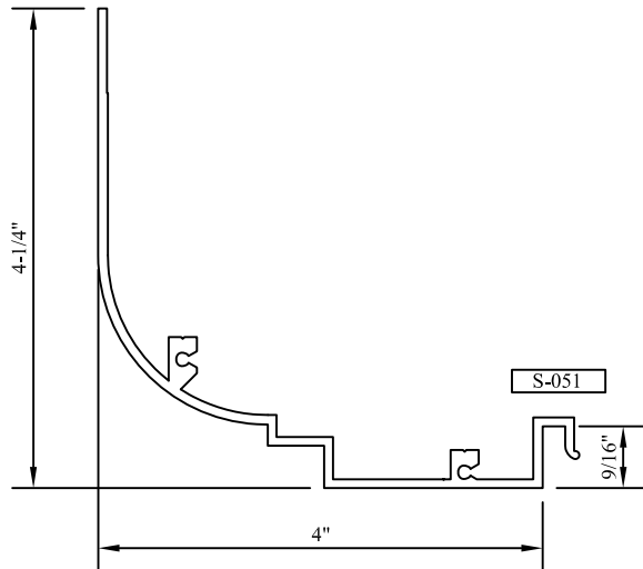
"U" HEAD/JAMB PANNING U
