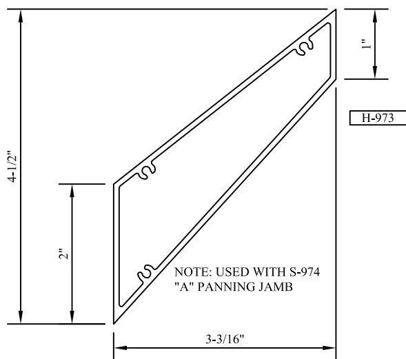
PANNING SPREADER BAR
