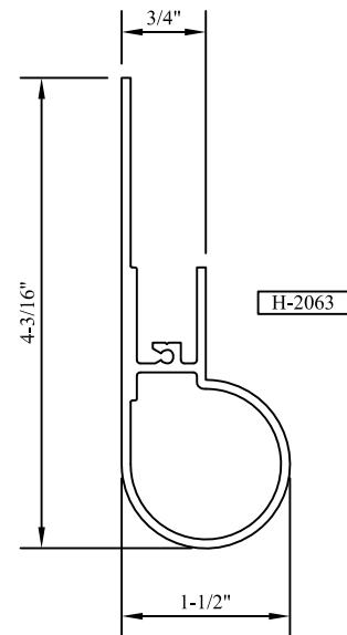
EXTERIOR TRIM PANNING
