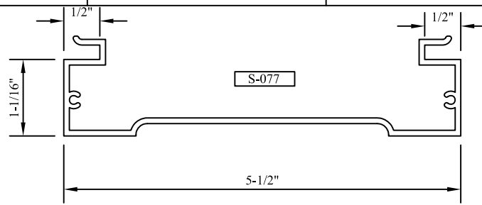
5-1/2" SPECIAL PANNING MULLION
