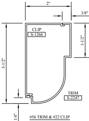
#56 TRIM
