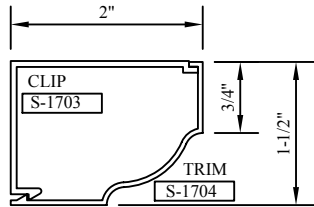
#41 TRIM & #41 CLIP
