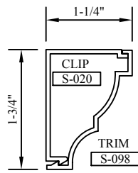
#11 TRIM & #6 CLIP
