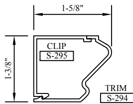
#17 TRIM & #17 CLIP
