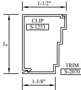
#2A TRIM & #2 CLIP
