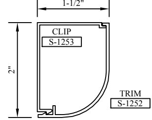
DECO SILL TRIM & #2 TRIM CLIP
