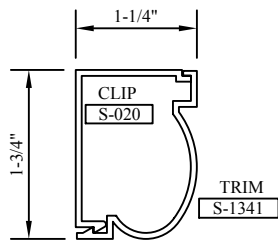
#23 TRIM & #6 CLIP
