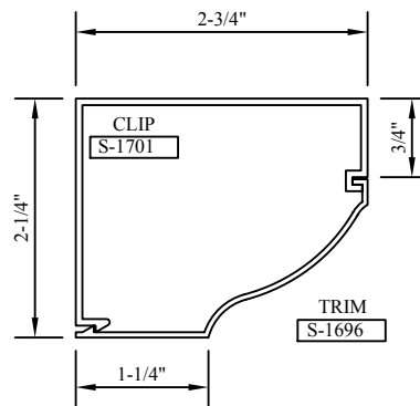
#38 TRIM & #40 CLIP
