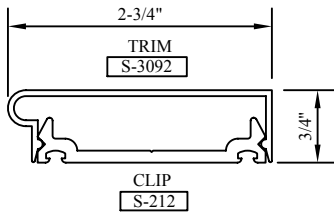
#85 TRIM & PRESSURE PLATE
