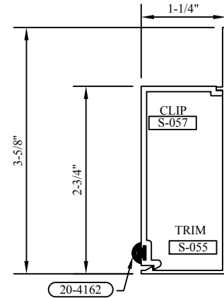
#7A TRIM & #7A PRESSURE CLIP #7A TRIM
