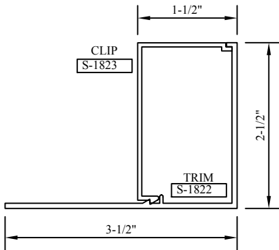
#43 TRIM & #43 CLIP #43 TRIM
