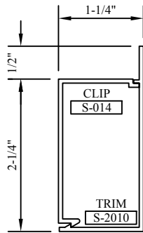
#3B TRIM & #3 CLIP #3B TRIM
