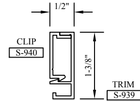
TILT STOP TRIM & TILT STOP CLIP TILT STOP TRIM
