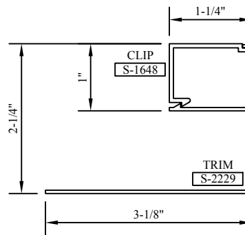
#55 TRIM & #36 CLIP #55 TRIM
