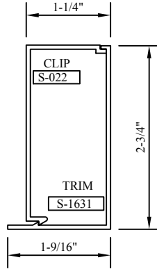
#35 TRIM & #7 CLIP #35 TRIM
