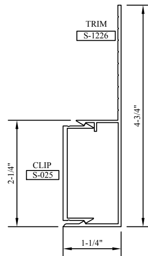
#7B EXTENSION TRIM & .750 HGH STOOL CLIP #7B TRIM
