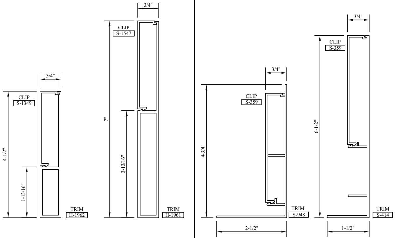
4 1/2" INTERIOR TRIM
