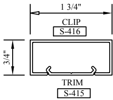
3/4" x 1-3/4" TRIM & CLIP
