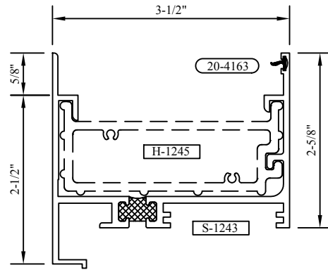
10 PSF SUBSILL S-1243
