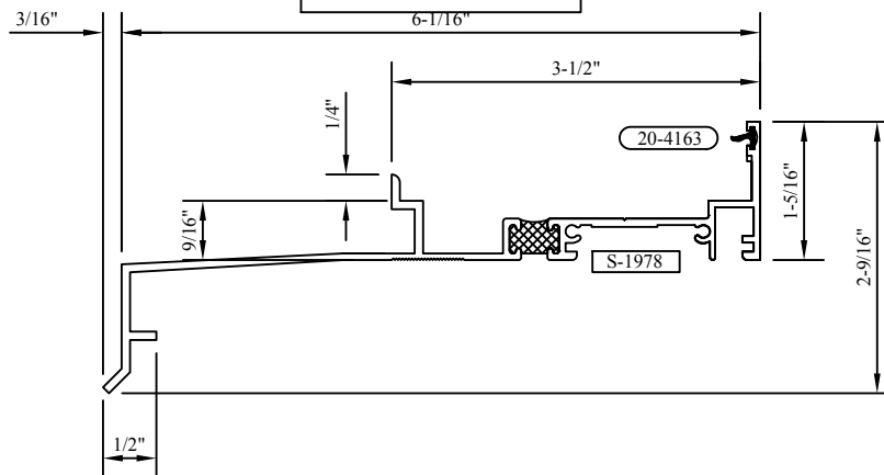
6.24 PSF SUBSILL S-1978
