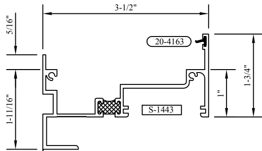
8 PSF SUBSILL S-1443
