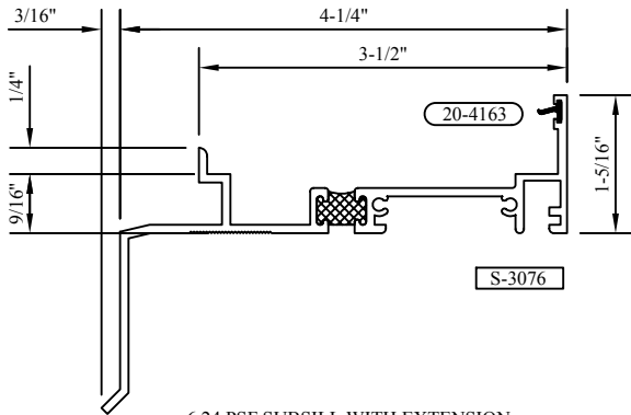
6.24 PSF SUBSILL WITH EXTENSION S-3076
