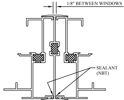
STACK MULLION (VERTICAL ONLY)
