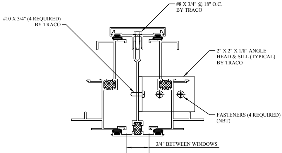
3 PIECE MULLION (VERTICAL ONLY)
