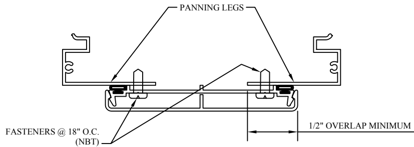
MULLION PRESSURE PLATE & COVER (VERTICAL OR HORIZONTAL)
