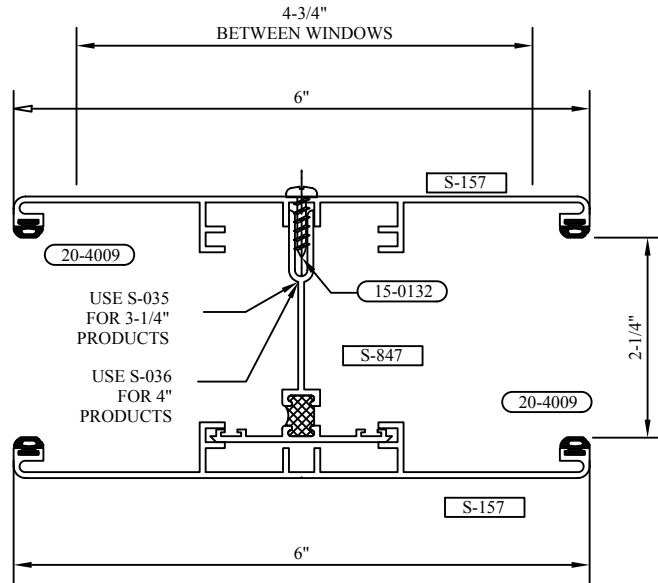
6" PARTITION MULLION S-157
