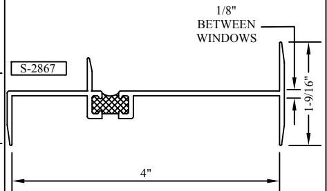
4" OFFSET STACK MULLION S-2867
