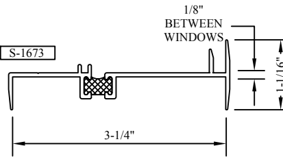
OFFSET STACK MULLION S-1673
