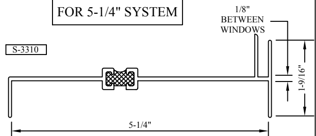
5-1/4" OFFSET STACK MULLION S-3310
