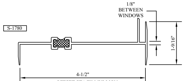
OFFSET STACK MULLION S-1780
