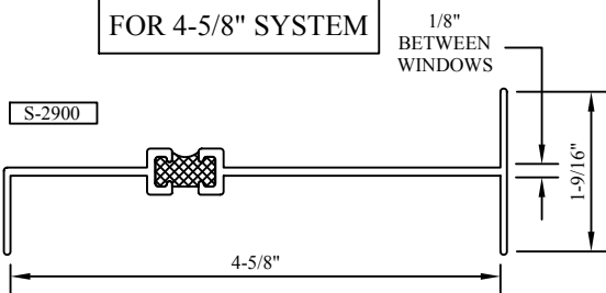
4-5/8" OFFSET STACK MULLION S-2900
