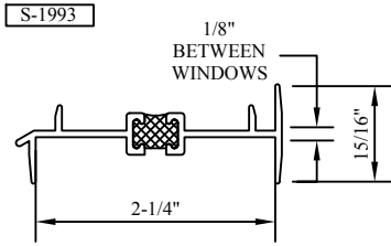
OFFSET STACK MULLION S-1993
