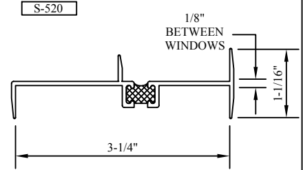
OFFSET STACK MULLION S-520
