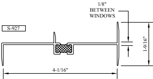
OFFSET STACK MULLION S-927
