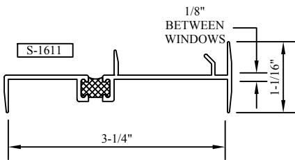
OFFSET STACK MULLION S-1611
