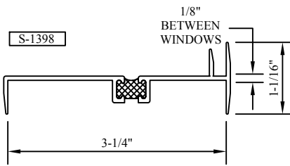
OFFSET STACK MULLION S-1398
