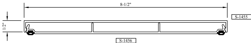
8-1/2" MULLION BASE & COVER S-1455 / S-1456
