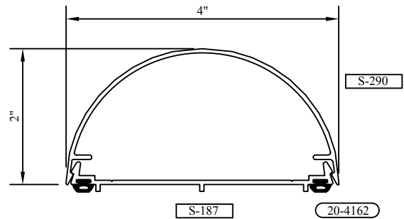
BULLNOSE MULLION COVER S-2907 / S-187
