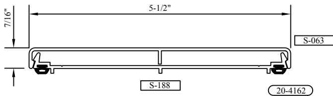
5-1/2" MULLION BASE & COVER S-063 / S-188
