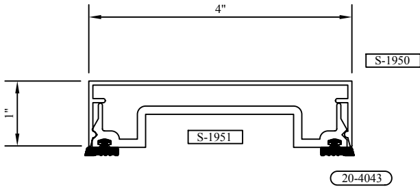
4" COVER W/ PLATE S-1950 / S-1951
