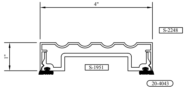
4" MULLION COVER & PLATE S-2248 / S-1951
