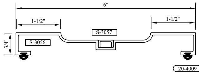
6" MULLION & COVER S-3056 / S-3057
