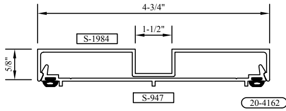
MULLION BASE & COVER S-1984 / S-947
