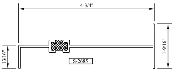
STACK MULLION S-2685
