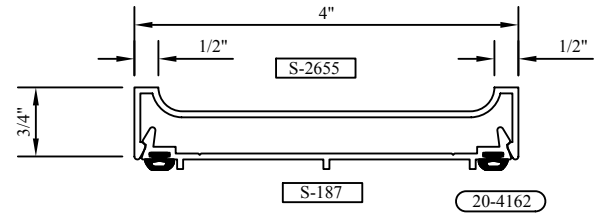
MULLION BASE & COVER S-2655 / S-187
