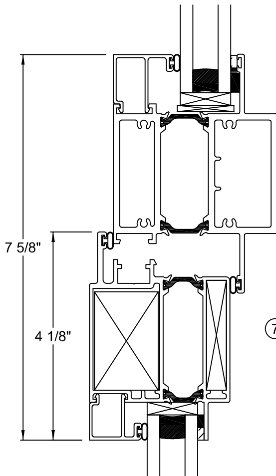
⑥ VERTICAL INTEGRAL MULLION (PANEL/FIXED)
