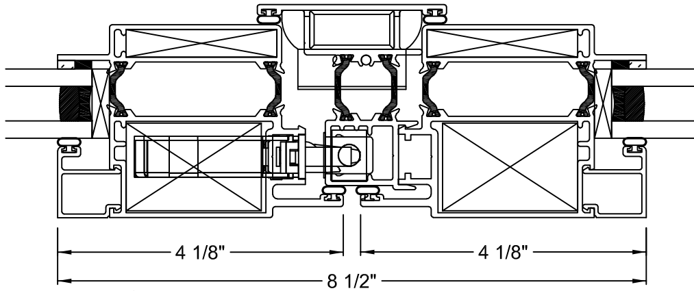
⑤ VERTICAL INTEGRAL MULLION (PANEL/PANEL)
