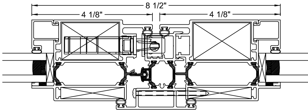
⑤ VERTICAL INTEGRAL MULLION (PANEL/PANEL)
