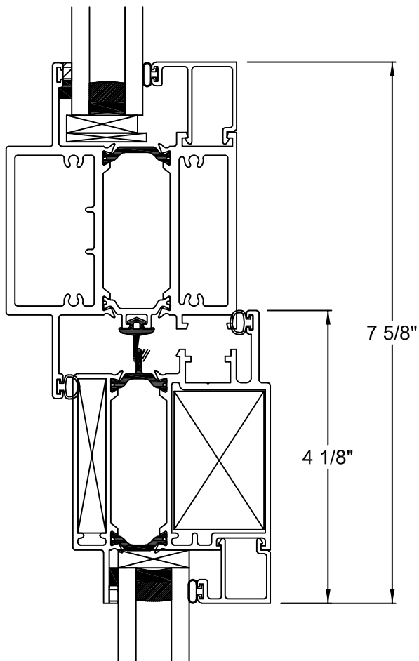
⑦ HORIZONTAL INTEGRAL MULLION (FIXED/PANEL)
