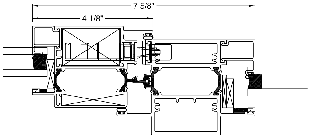
⑥ VERTICAL INTEGRAL MULLION (PANEL/FIXED)
