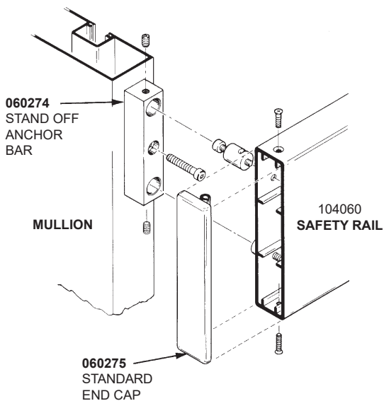
RAILING MOUNTED ON FACE OF MULLION
