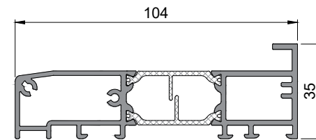
3002 723 Cill profile 6400mm stock length
