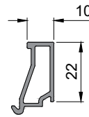
170 315 Glazing bead 6000mm stock length
