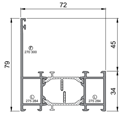
3001 094 Integral 34mm outer frame 5000mm stock length
