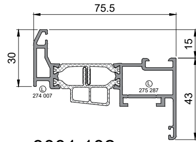
3001 102 Integral TBT vent 5000mm stock length
