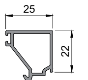
694 320 Glazing bead 6400mm stock length
