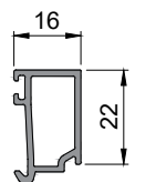
694 317 Glazing bead 6400mm stock length
