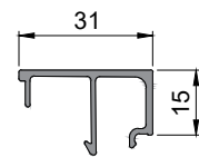
170 358 Glazing bead 6000mm stock length
