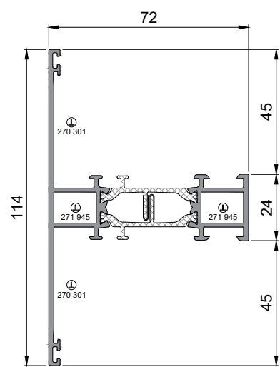
3001 099 Integral 24mm Muntin 5000mm stock length
