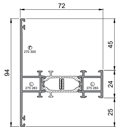
3001 097 Integral 24mm Muntin 5000mm stock length
