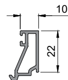
694 315 Glazing bead 6400mm stock length
