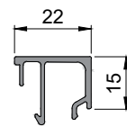
171 338 Glazing bead 6000mm stock length
